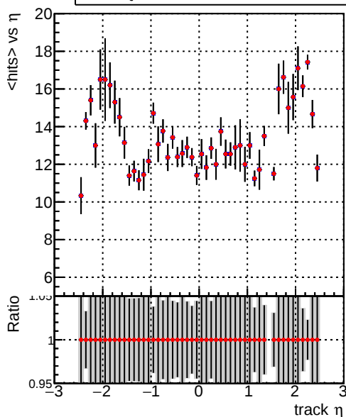
— DQM_V0001_R000000001_Global_mkFit100i0_RECO — DQM_V0001_R000000001_Global_mkFit1000mod_RECO
