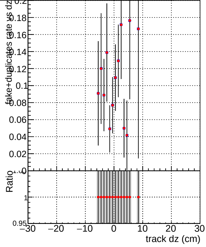
DQM_V0001_R0000000001_Global_mkFiti100i0_RECO DQM_V0001_R0000000001_Global_mkFiti1000mod_RECO
