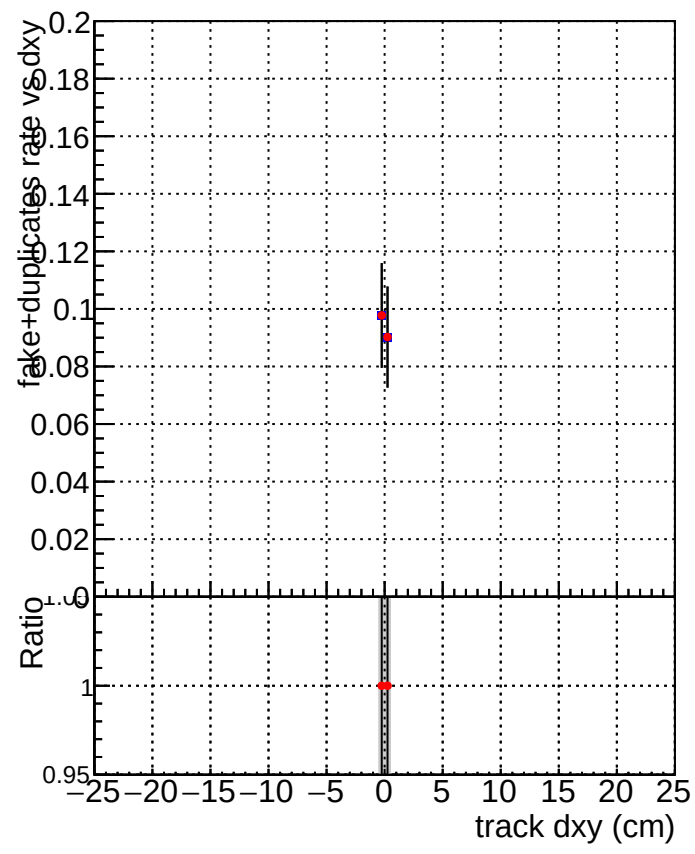
DQM_V0001_R0000000001_Global_mkFiti100i0_RECO DQM_V0001_R0000000001_Global_mkFiti1000mod_RECO
