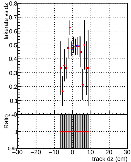
Fake rate vs dz Legend: Global mkFit1000i0 RECO (Blue dots) Global mkFit1000mod RECO (Red dots)
