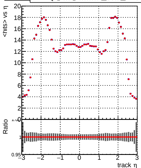
— DQM_V0001_R000000001_Global_mkFit1000i0_RECO — DQM_V0001_R000000001_Global_mkFit1000mod_RECO
