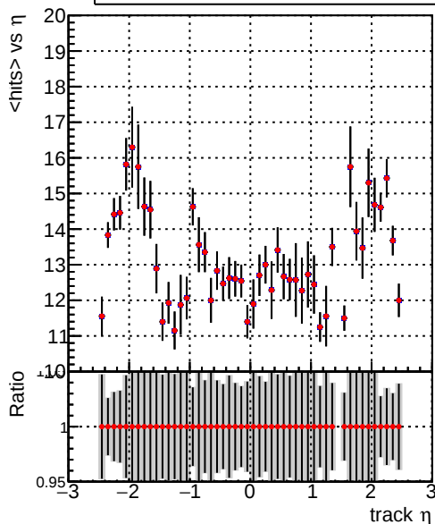
mean hit — DQM_V0001_R000000001_Global_mkFit100i0_RECO — DQM_V0001_R000000001_Global_mkFit1000mod_RECO
