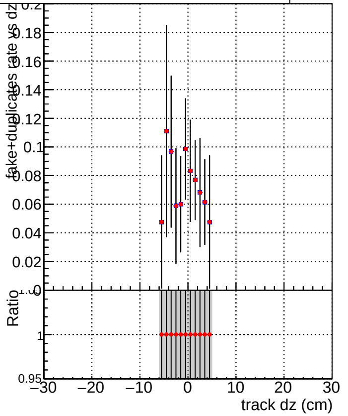
DQM_V0001_R0000000001_Global_mkFiti100i0_RECO DQM_V0001_R0000000001_Global_mkFiti1000mod_RECO
