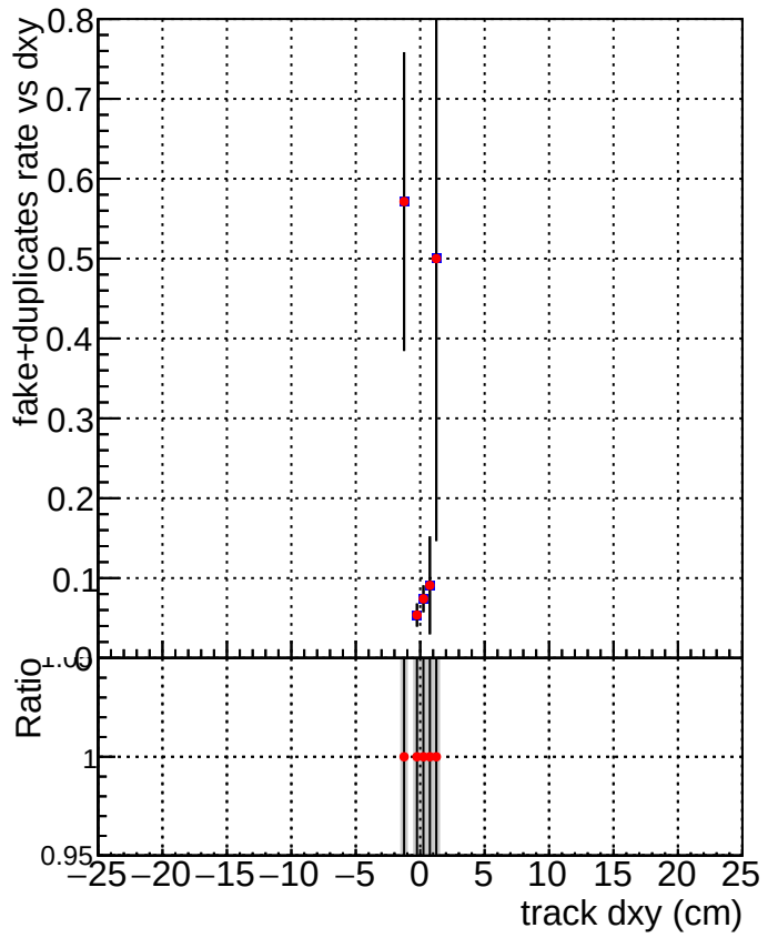
DQM_V0001_R0000000001_Global_mkFiti100i0_RECO DQM_V0001_R0000000001_Global_mkFiti1000mod_RECO
