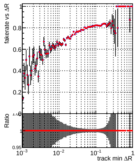
—●— DQM_V0001_R000000001_Global_mkFiti100i0_RECO —●— DQM_V0001_R000000001_Global_mkFiti1000mod_RECO
