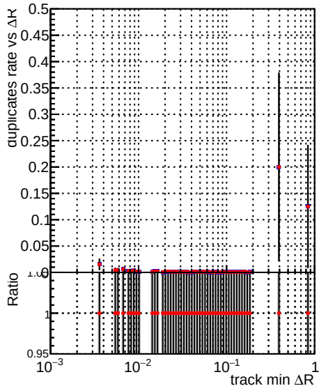
—●— DQM_V0001_R000000001_Global_mkFiti100i0_RECO —●— DQM_V0001_R000000001_Global_mkFiti1000mod_RECO
