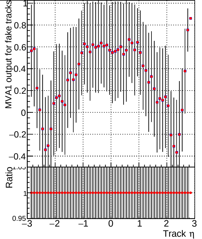
MVA1 of associated tracks (recoToSim) vs. track \eta ■ DQM_V0001_R000000001_Global_mkFiti100i0_RECO ● DQM_V0001_R000000001_Global_mkFiti1000mod_RECO
