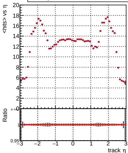
— DQM_V0001_R000000001_Global_mkFit1000i0_RECO — DQM_V0001_R000000001_Global_mkFit1000mod_RECO
