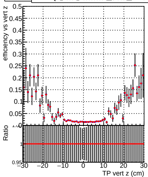
Efficiency vs TP vert z (cm) — DQM_V0001_R000000001_Global_mkFiti1000i0_RECO — DQM_V0001_R000000001_Global_mkFiti1000mod_RECO
