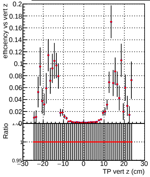
Efficiency vs. TP vert z — DQM_V0001_R0000000001_Global_mkFit1000i0_RECO — DQM_V0001_R0000000001_Global_mkFit1000mod_RECO
