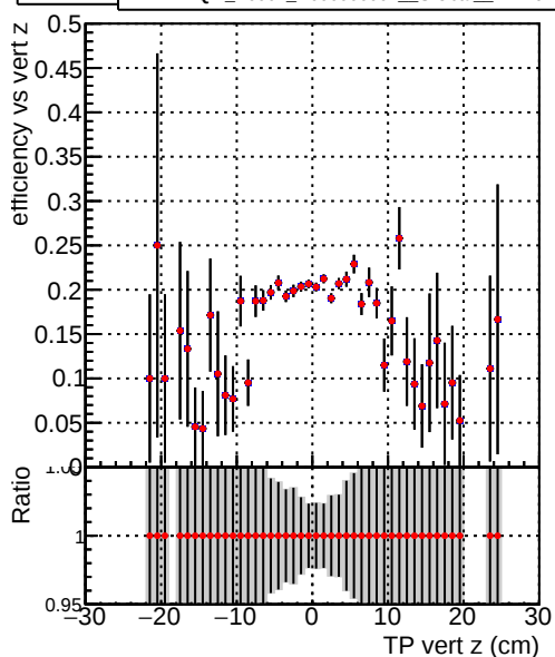
Efficiency vs vert z — DQM_V0001_R000000001_Global_mkFit1000i0_RECO — DQM_V0001_R000000001_Global_mkFit1000mod_RECO
