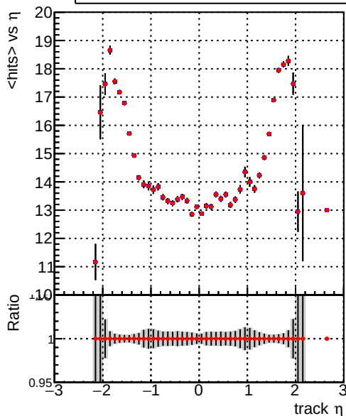
mean hits vs \eta — DQM_V0001_R000000001_Global_mkFit100i0_RECO — DQM_V0001_R000000001_Global_mkFit1000mod_RECO
