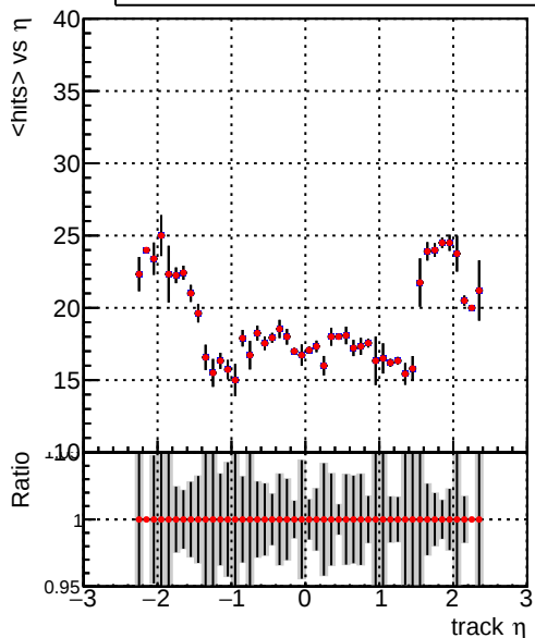
mean hits — DQM_V0001_R000000001_Global_mkFit100i0_RECO — DQM_V0001_R000000001_Global_mkFit1000mod_RECO
