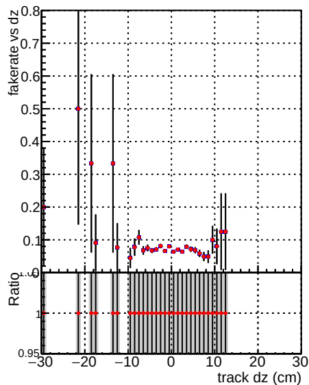
DQM_V0001_R000000001_Global_mkFiti100i0_RECO Fake rate vs d DQM_V0001_R000000001_Global_mkFiti1000mod_RECO
