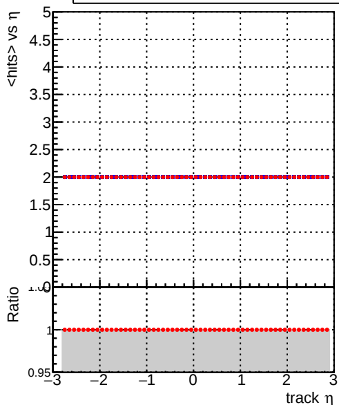
mean hits vs \eta Legend: DQM_V0001_R000000001_Global_mkFitQCDi1_RECO (blue line), DQM_V0001_R000000001_Global_mkFitQCDmod_RECO (red line)
