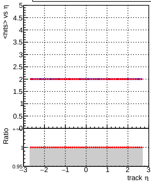
mean hits DQM_V0001_R000000001_Global_mkFitQCDi1_RECO DQM_V0001_R000000001_Global_mkFitQCDmod_RECO
