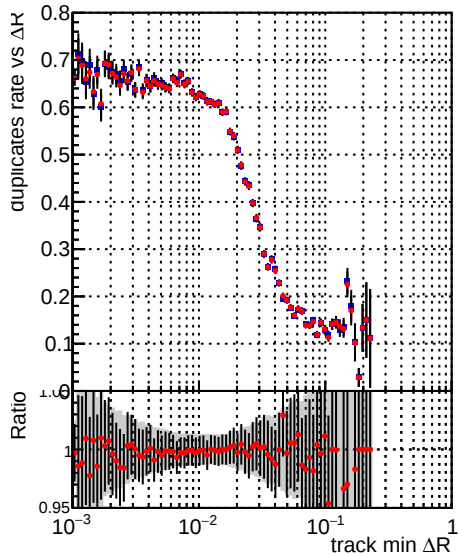
—●— DQM_V0001_R000000001_Global_mkFitQCDi1_RECO —●— DQM_V0001_R000000001_Global_mkFitQCDmod_RECO
