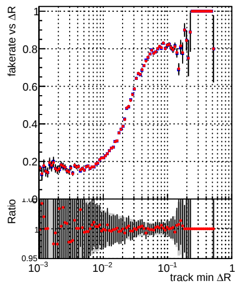
—●— DQM_V0001_R000000001_Global_mkFitQCDi1_RECO —●— DQM_V0001_R000000001_Global_mkFitQCDmod_RECO
