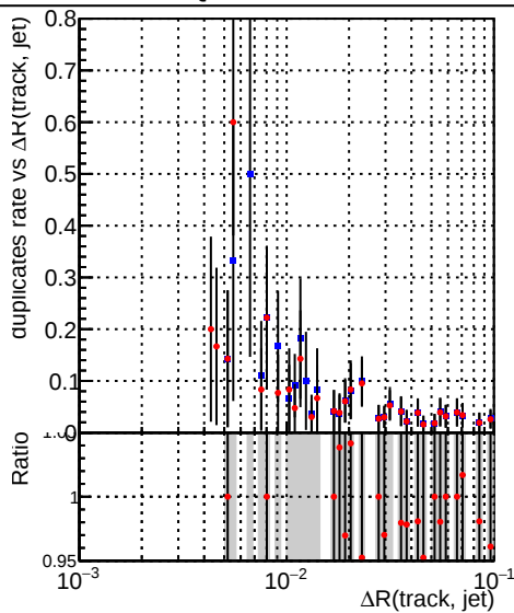
—●— DQM_V0001_R000000001_Global_mkFitQCDi1_RECO —●— DQM_V0001_R000000001_Global_mkFitQCDmod_RECO
