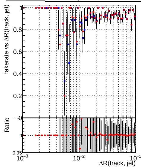
—●— DQM_V0001_R000000001_Global_mkFitQCDi1_RECO —●— DQM_V0001_R000000001_Global_mkFitQCDmod_RECO
