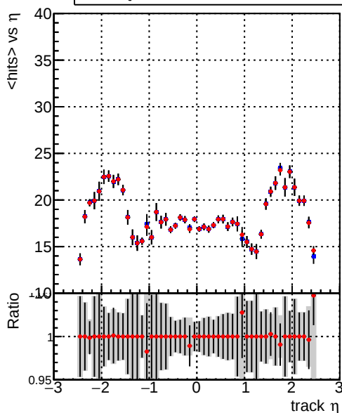
— DQM_V0001_R000000001_Global_mkFitQCDi1_RECO — DQM_V0001_R000000001_Global_mkFitQCDmod_RECO
