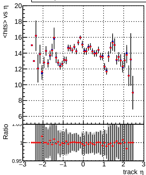
— DQM_V0001_R000000001_Global_mkFitQCDi1_RECO — DQM_V0001_R000000001_Global_mkFitQCDmod_RECO
