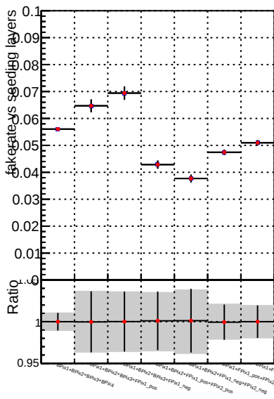
Fake rate vs. —●— DQM_V0001_R000000001_Global_mkFitQCDi1_RECO —●— DQM_V0001_R000000001_Global_mkFitQCDmod_RECO
