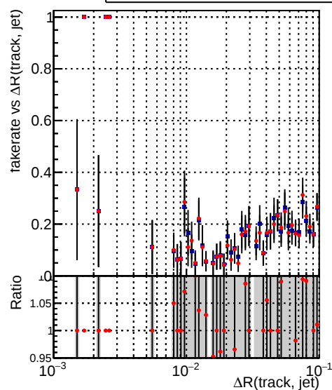
—●— DQM_V0001_R000000001_Global_mkFitQCDi1_RECO —●— DQM_V0001_R000000001_Global_mkFitQCDmod_RECO
