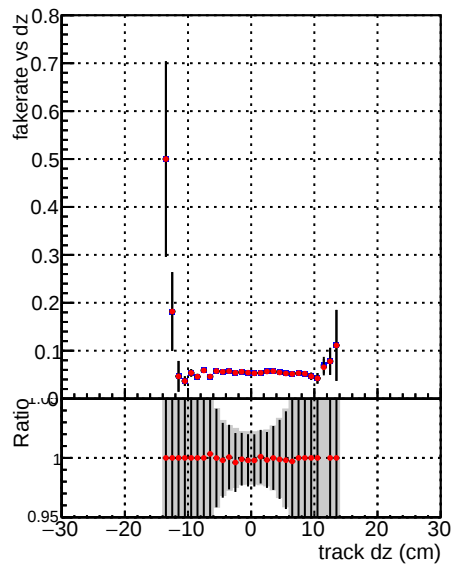
—●— DQM V0001_R0000000001 Global mkFitQCDi1 RECO —●— DQM V0001_R0000000001 Global mkFitQCDmod RECO
