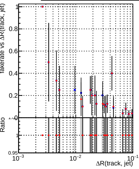
Legend: \blacksquare DQM_V0001_R000000001_Global_mkFitQCDi1_RECO \bullet DQM_V0001_R000000001_Global_mkFitQCDmod_RECO
