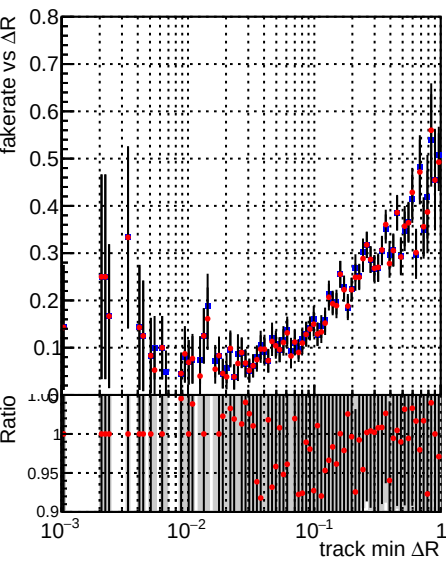
Legend: \blacksquare DQM_V0001_R000000001_Global_mkFitQCDi1_RECO \bullet DQM_V0001_R000000001_Global_mkFitQCDmod_RECO
