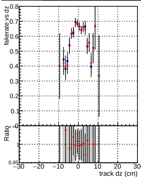
—●— DQM V0001_R000000001 Global mkFitQCDi1 RECO —●— DQM V0001_R000000001 Global mkFitQCDmod RECO
