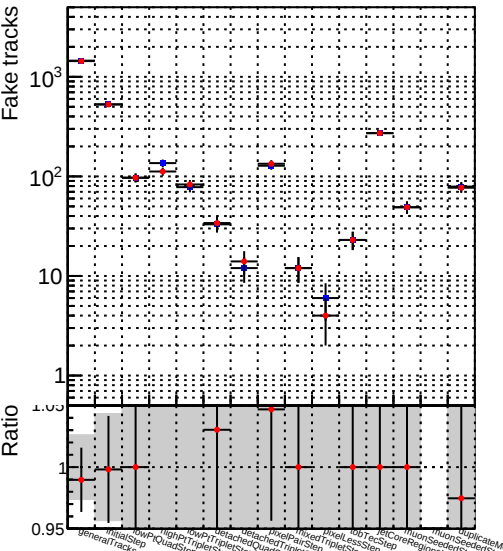
Number 1 DQM_V0001_R000000001_Global_mkFitQCDmod_RECO
