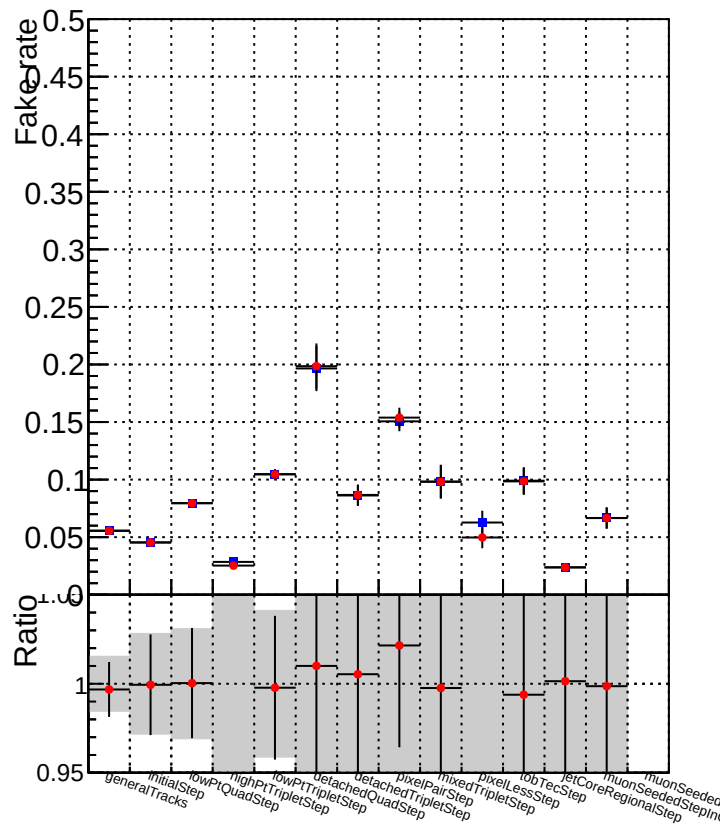
DQM_V0001_R0000000001_Global_mkFitQCDi1_RECO DQM_V0001_R0000000001_Global_mkFitQCDmod_RECO
