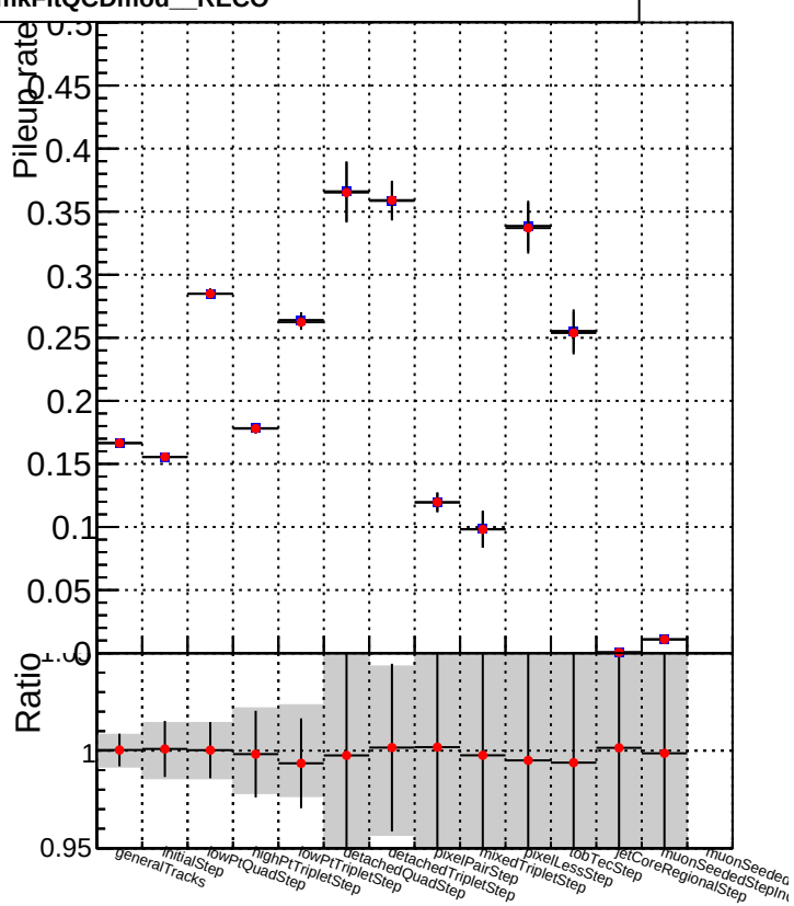
DQM_V0001_R0000000001_Global_mkFitQCDi1_RECO DQM_V0001_R0000000001_Global_mkFitQCDmod_RECO
