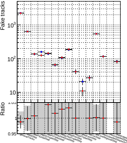
Number —●— DQM_V0001_R000000001 Global mkFitQCDmod RECO
