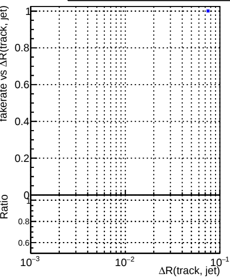
Legend: —■— DQM_V0001_R000000001_Global_mkFitQCDi1_RECO —●— DQM_V0001_R000000001_Global_mkFitQCDmod_RECO
