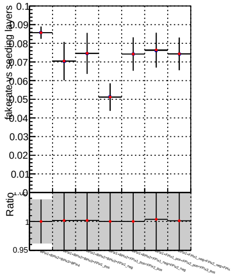
Fake rate vs. DQM V0001_R000000001 Global mkFitQCDi1 RECO DQM V0001_R000000001 Global mkFitQCDmod RECO
