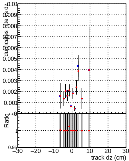
al_mkFitQCDmod_RECO
