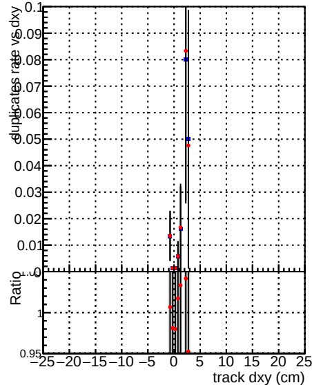
al_mkFitQCDmod_RECO
