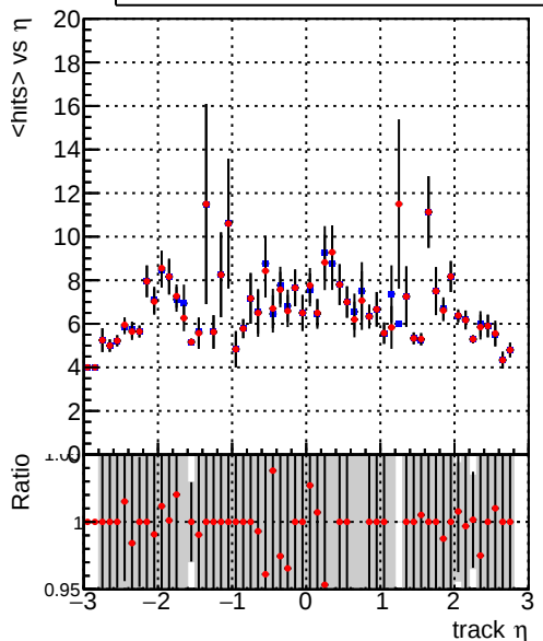
mean hits — DQM_V0001_R000000001_Global_mkFitQCDi1_RECO — DQM_V0001_R000000001_Global_mkFitQCDmod_RECO
