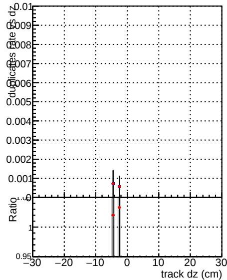
—●— DQM_V0001_R0000000001_Global_mkFitQCDi1_RECO —●— DQM_V0001_R0000000001_Global_mkFitQCDmod_RECO
