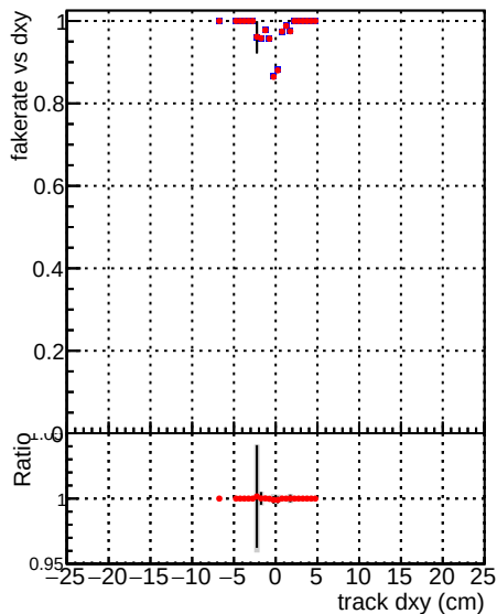
Fake rate vs d DQM_V0001_R000000001_Global_mkFitQCD1_RECO DQM_V0001_R000000001_Global_mkFitQCDmod_RECO
