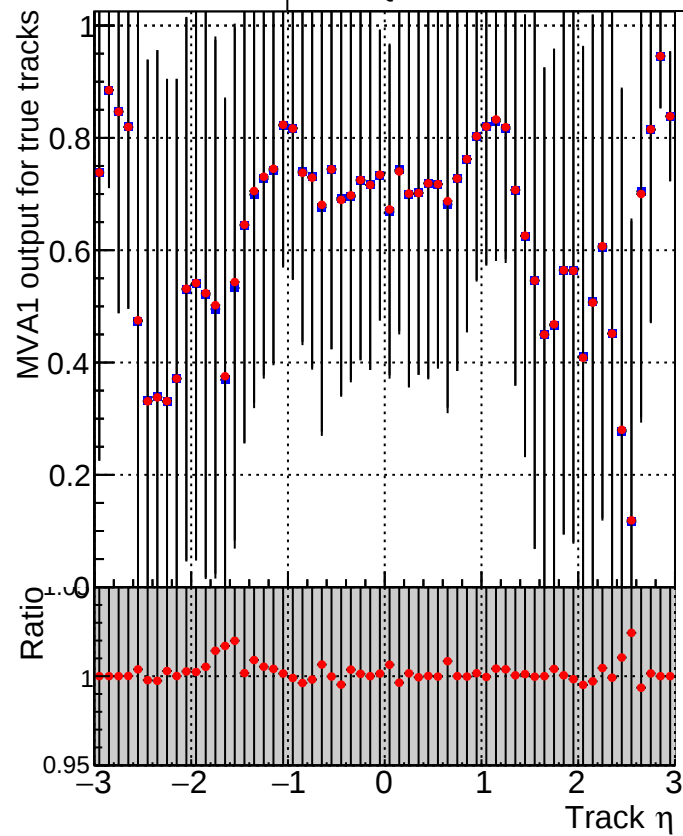
MVA1 of associated tracks (recoToSim) vs. track \eta ■ DQM_V0001_R000000001_Global_mkFitQCDi1_RECO ● DQM_V0001_R000000001_Global_mkFitQCDmod_RECO
