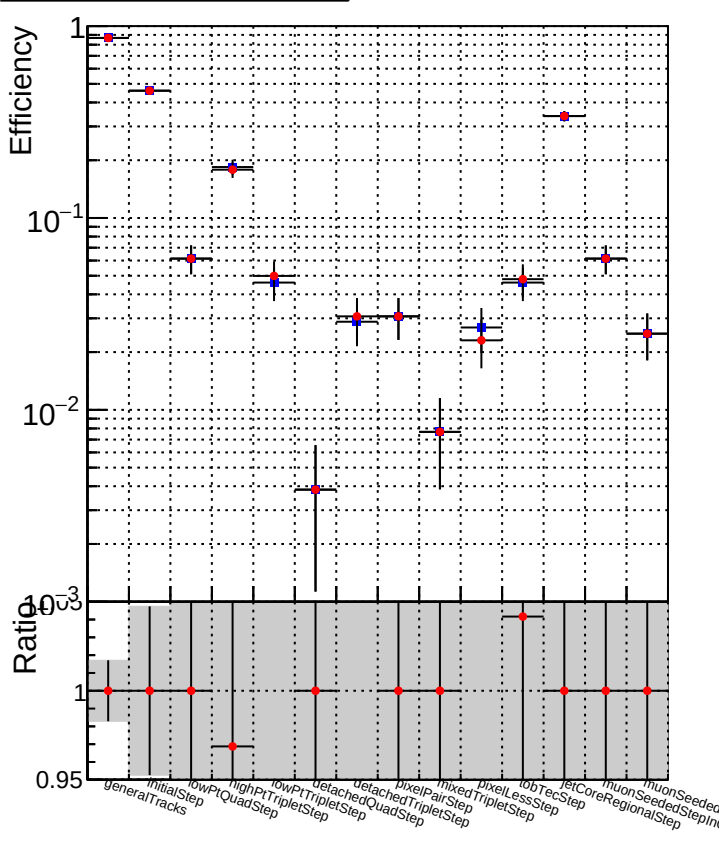
DQM_V0001_R000000001_Global_mkFitQCDi1_RECO DQM_V0001_R000000001_Global_mkFitQCDmod_RECO
