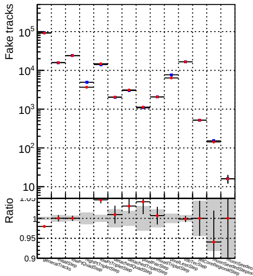
Number of tracks vs collection Legend: DQM_V0001_R000000001_Global_mkFitQCDi1_RECO DQM_V0001_R000000001_Global_mkFitQCDmod_RECO
