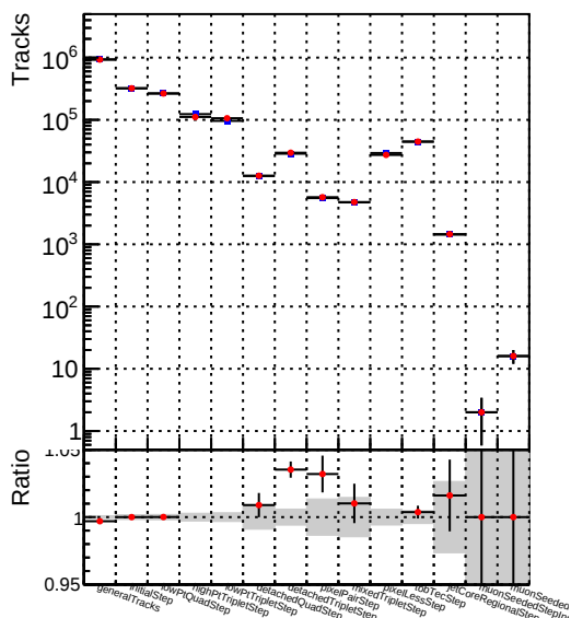
DQM_V0001_R000000001_Global_mkFitQCDi1_RECO
