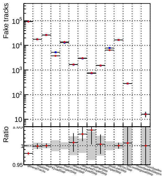
Number —●— DQM_V0001_R000000001_Global_mkFitQCDmod_RECO
