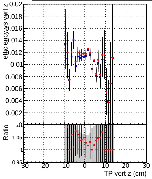
Efficiency vs. TP vert z (cm) — DQM_V0001_R000000001_Global_mkFitQCDi1_RECO — DQM_V0001_R000000001_Global_mkFitQCDmod_RECO
