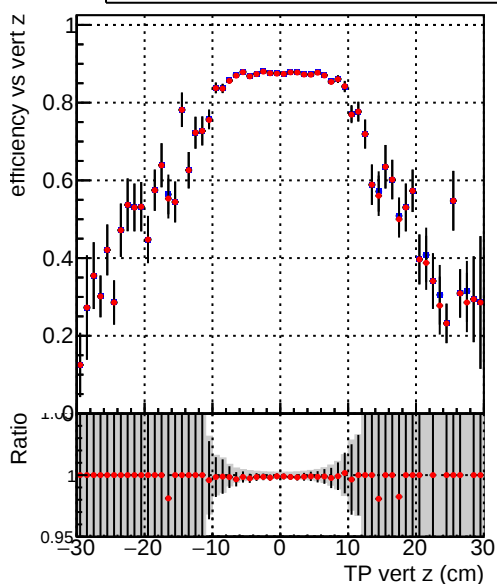
Efficiency vs vert z —●— DQM_V0001_R0000000001_Global_mkFitQCDi1_RECO —●— DQM_V0001_R0000000001_Global_mkFitQCDmod_RECO
