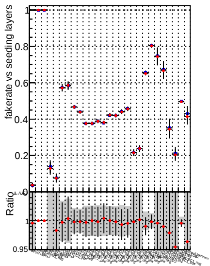
Fake rate vs. —●— DQM V0001_R000000001 Global mkFitQCDi1_RECO —●— DQM V0001_R000000001 Global mkFitQCDmod_RECO
