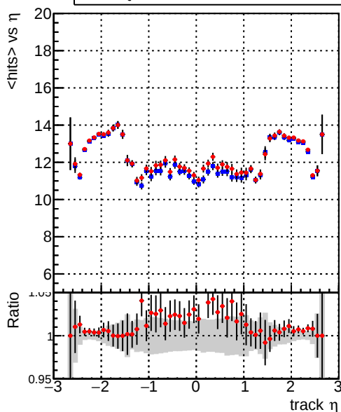
mean hits vs \eta — DQM_V0001_R000000001_Global_mkFitQCDi1_RECO — DQM_V0001_R000000001_Global_mkFitQCDmod_RECO
