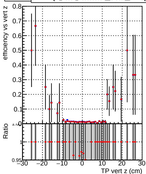
Efficiency vs TP vert z — DQM_V0001_R000000001_Global_mkFitQCDi1_RECO — DQM_V0001_R000000001_Global_mkFitQCDmod_RECO
