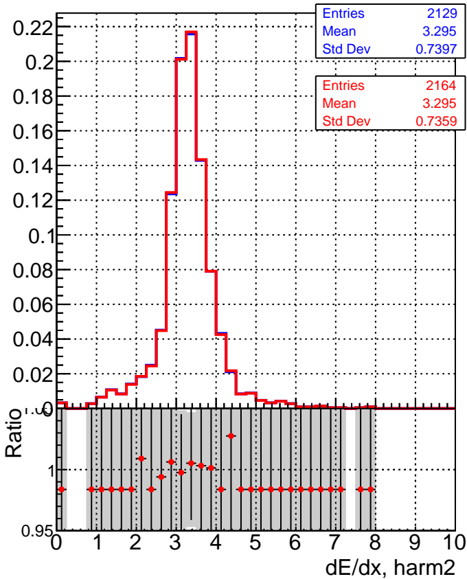
■ DQM_V0001_R000000001_Global_mkFitQCDi1_RECO ● DQM_V0001_R000000001_Global_mkFitQCDmod_RECO
