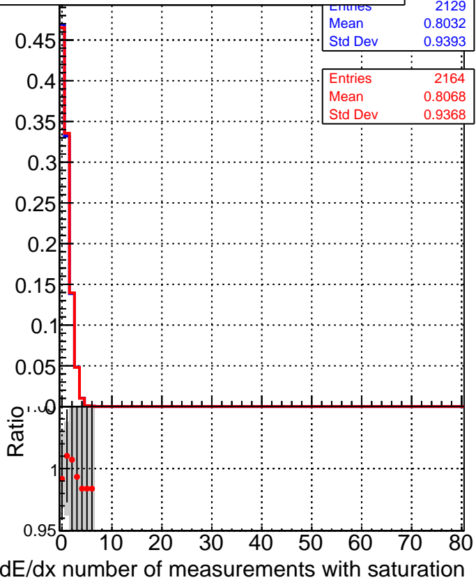
■ DQM_V0001_R000000001_Global_mkFitQCDi1_RECO ● DQM_V0001_R000000001_Global_mkFitQCDmod_RECO
