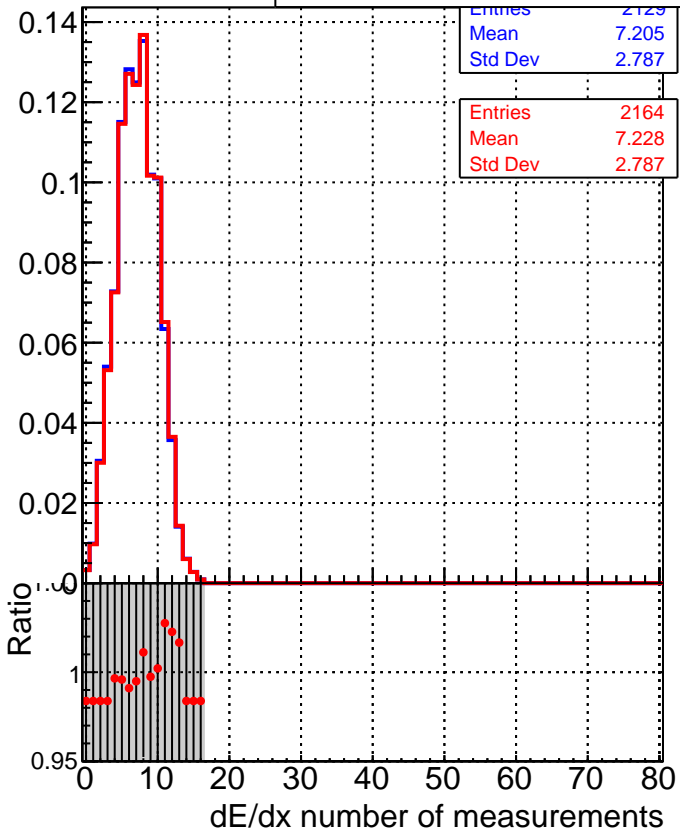
■ DQM_V0001_R000000001_Global_mkFitQCDi1_RECO ● DQM_V0001_R000000001_Global_mkFitQCDmod_RECO
