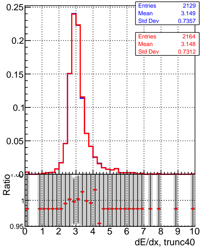
■ DQM_V0001_R000000001_Global_mkFitQCDi1_RECO ● DQM_V0001_R000000001_Global_mkFitQCDmod_RECO
