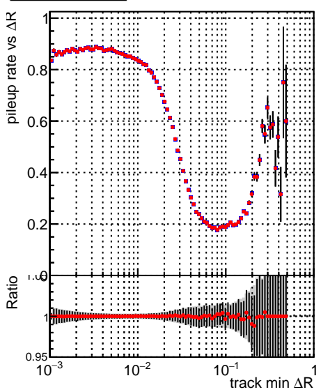
—•— DQM_V0001_R000000001_Global_CMSSW_orig —•— DQM_V0001_R000000001_Global_CMSSW_allchi2
