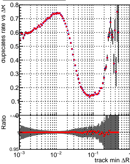
—•— DQM_V0001_R000000001_Global_CMSSW_orig —•— DQM_V0001_R000000001_Global_CMSSW_allchi2
