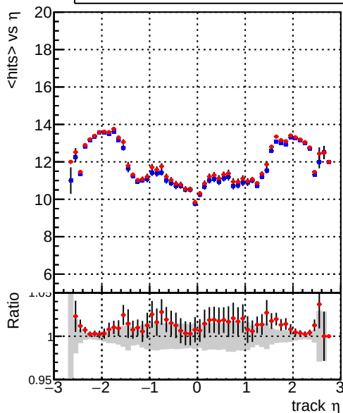
mean hit — DQM_V0001_R000000001_Global_CMSSW_orig — DQM_V0001_R000000001_Global_CMSSW_allchi2
