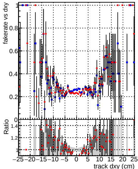
—●— DQM_V0001_R0000000001_Global_CMSSW_orig —●— DQM_V0001_R0000000001_Global_CMSSW_allchi2
