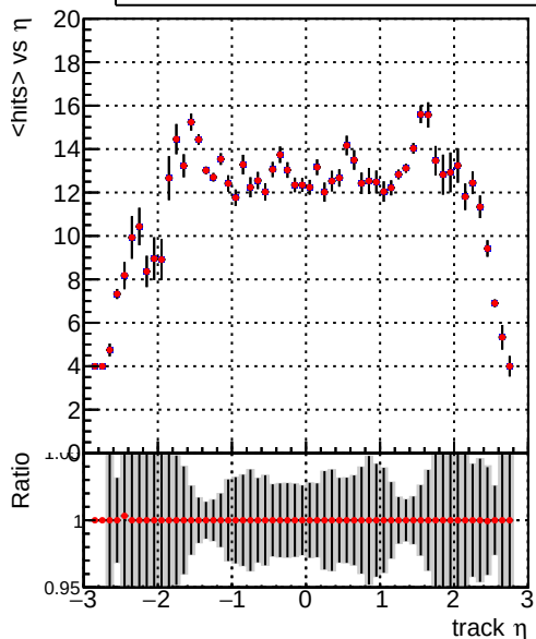
mean hit — DQM_V0001_R000000001_Global_CMSSW_orig — DQM_V0001_R000000001_Global_CMSSW_allchi2
