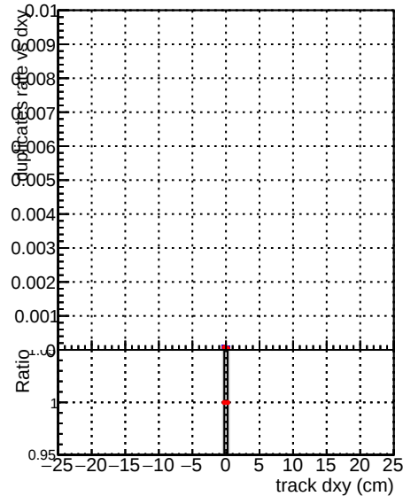
—●— DQM_V0001_R0000000001 Global CMSSW_orig —●— DQM_V0001_R0000000001 Global CMSSW_allchi2
