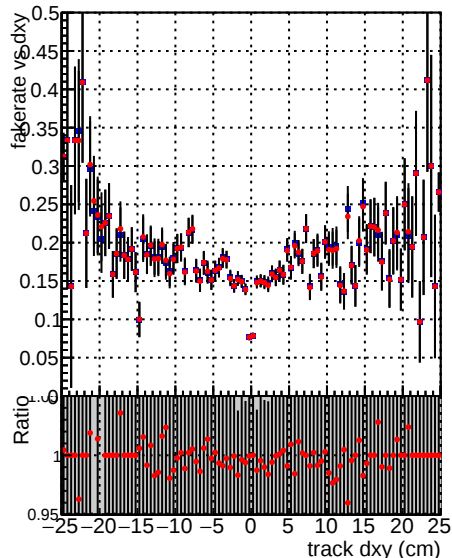
—●— DQM_V0001_R0000000001_Global_CMSSW_orig —●— DQM_V0001_R0000000001_Global_CMSSW_allchi2
